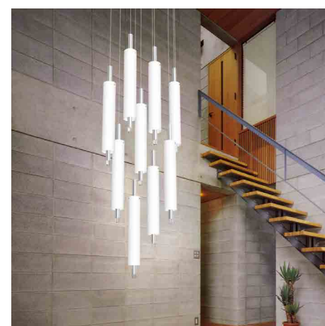
PINS DIMENSION - Ø4" X 2'-3" MATERIAL - ACRYLIC LIGHTING - LED
